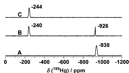
Figure 2. ^{199}\text{Hg} NMR spectra of solutions containing \alpha_3 DIV (2.93 mM) and ^{199}\text{Hg}(\text{NO}_3)_2 (0.8 equiv) at pH 5.8 (A), 7.4 (B), and 8.6 (C).
